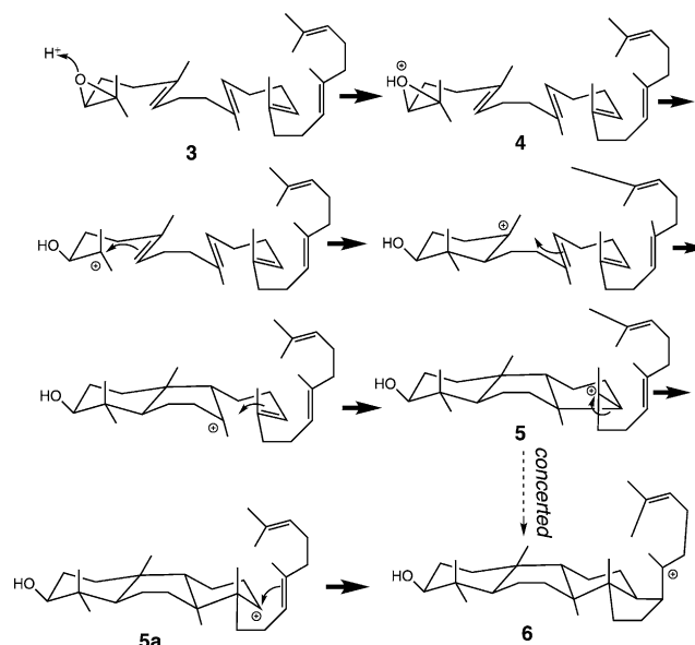
Scheme 2. Cyclization of squalene oxide ( 3 ) to the protosterol cation ( 6 ).
